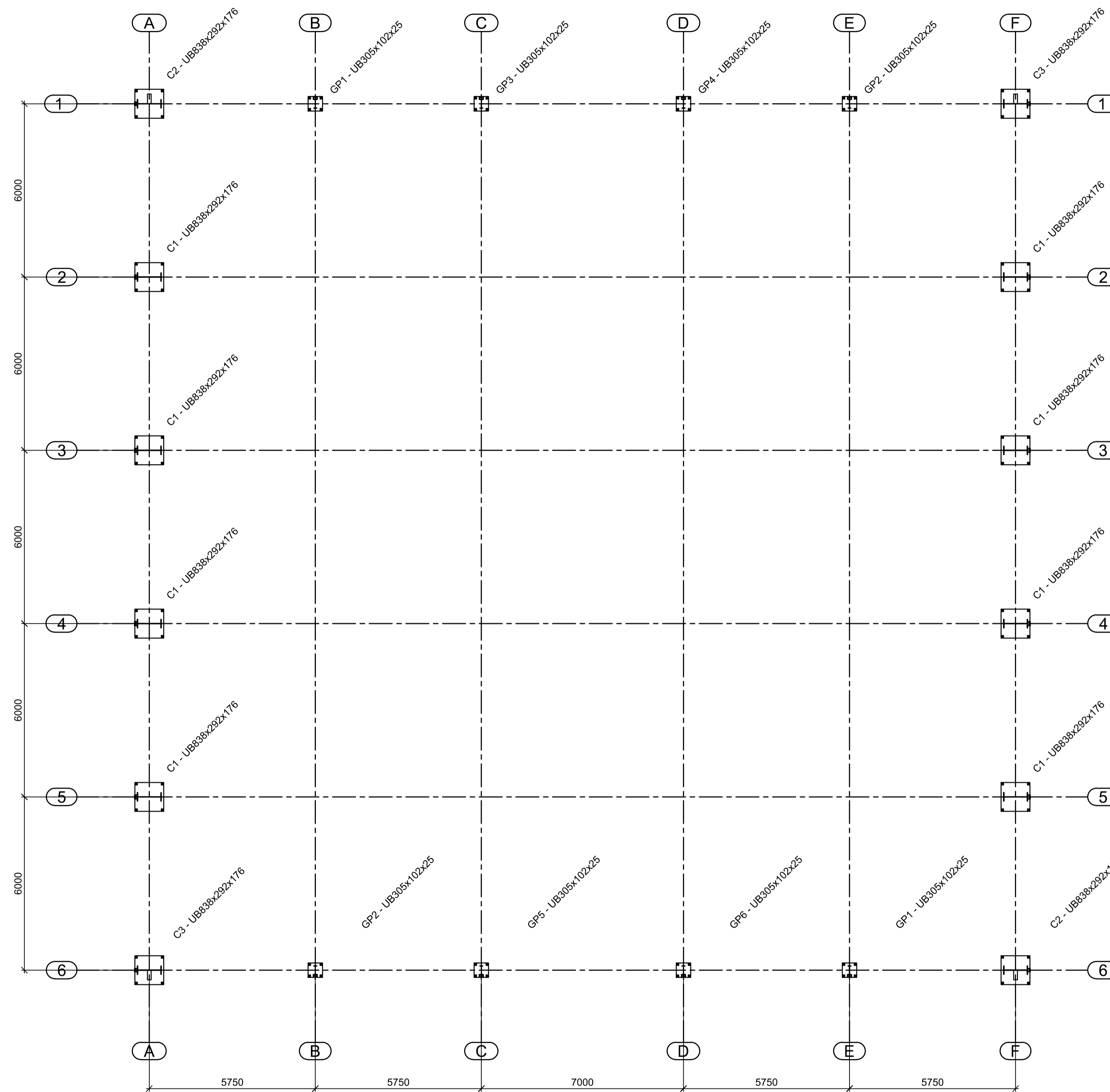
Base Plate Floor Plan
